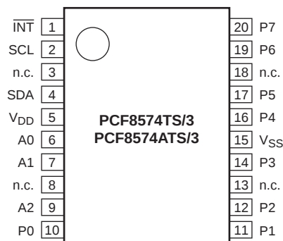
Fig 5. Pin configuration for SSOP20
