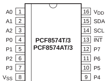
Fig 4. Pin configuration for SO16
